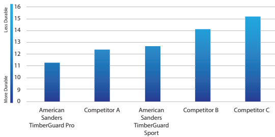
Taber Abrasion Test (Total mg Lost)
